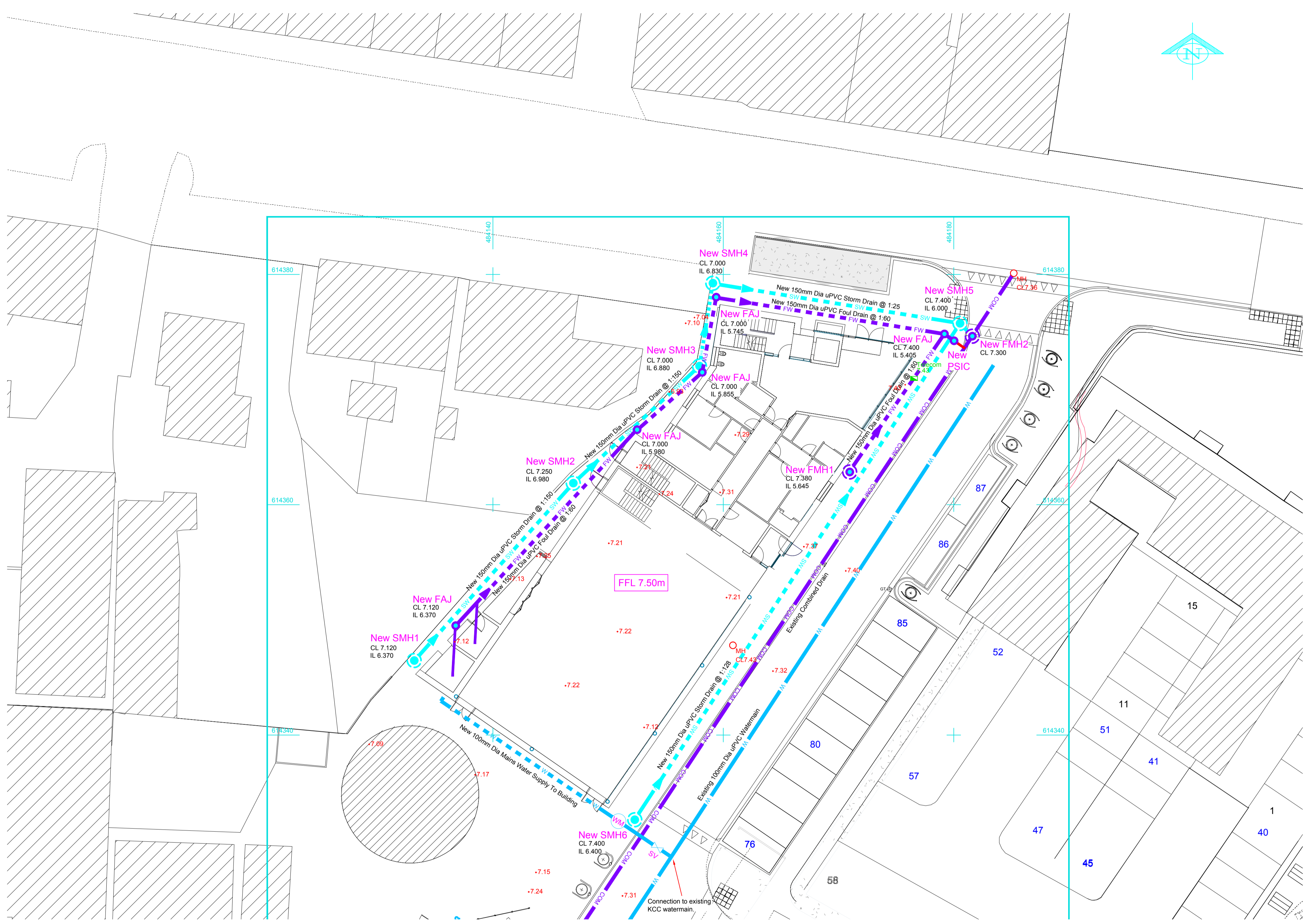
Proposed Drainage Layout Scale 1:200
